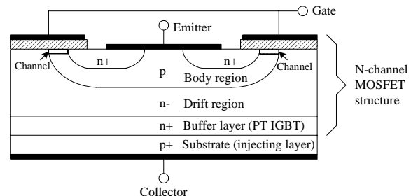
Figure 1 PT IGBT Cross Section
