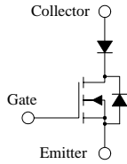
Figure 2 Simple IGBT Equivalent Circuit
