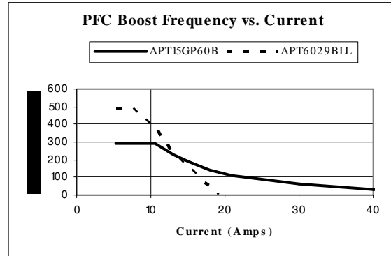
Figure 6 PFC Boost Frequency vs. Current
