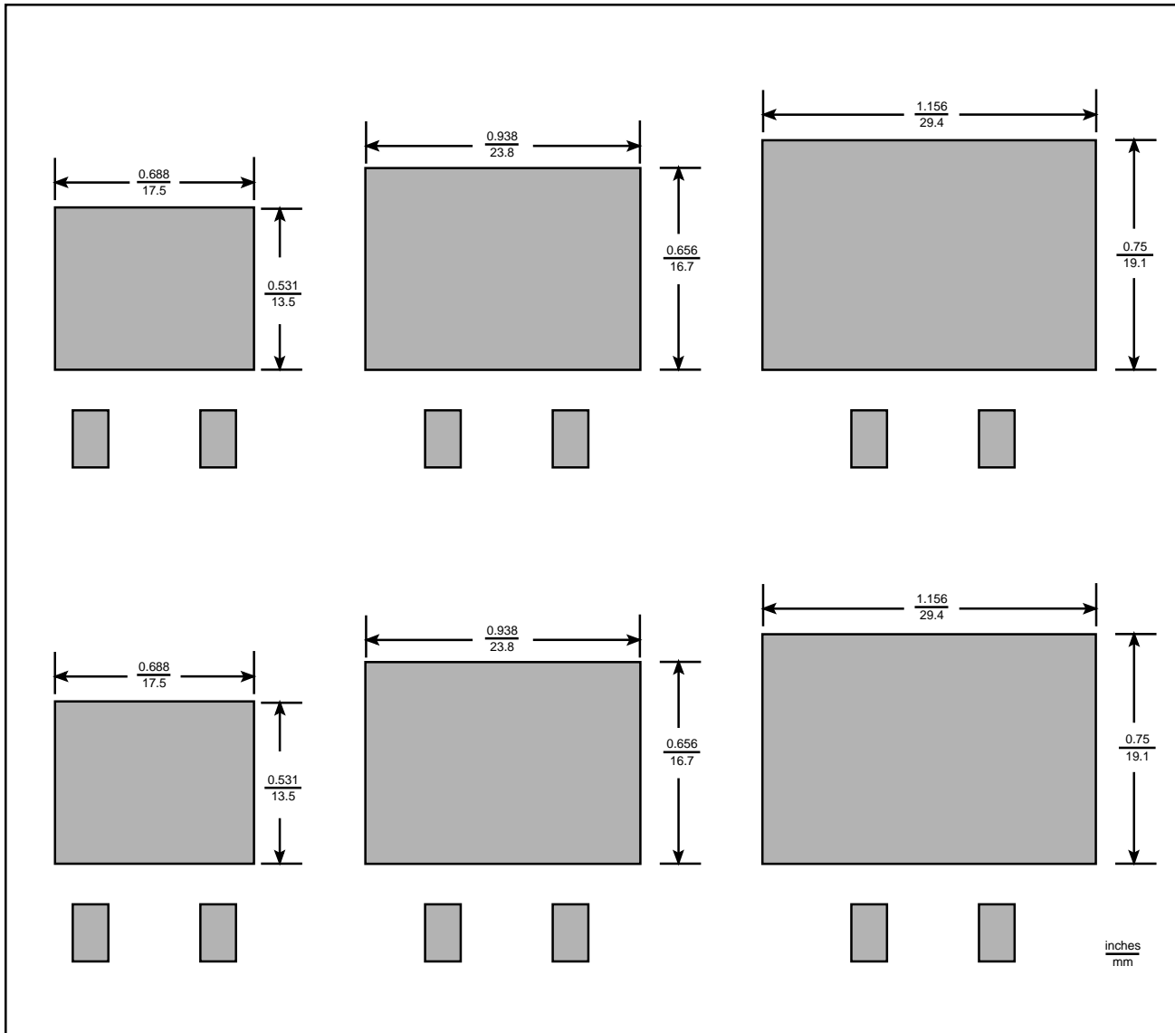
Figure 4. Printed Circuit Board Layout.
