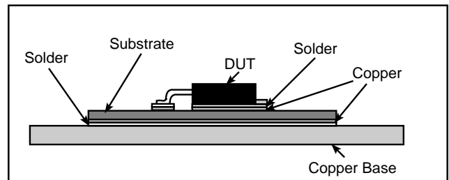
Figure 9. Cross Section of the D 3 PAK Mounted on the Substrate and Copper Base.
