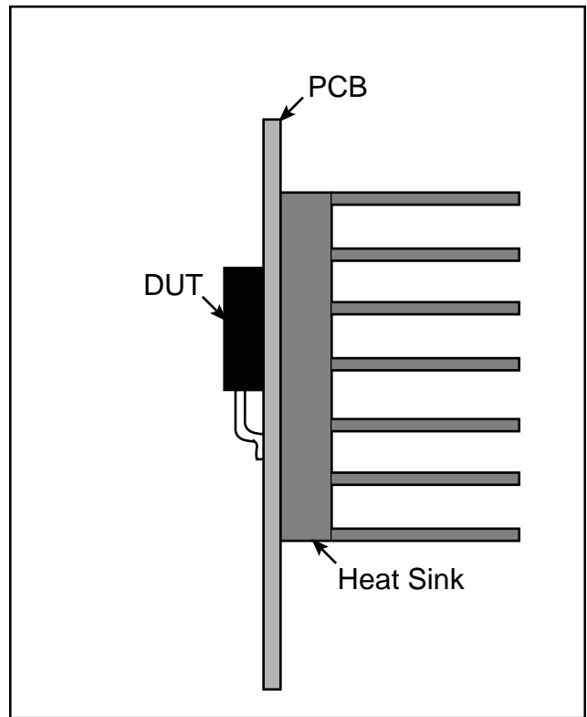
Figure 5. PCB With Heat Sink.
