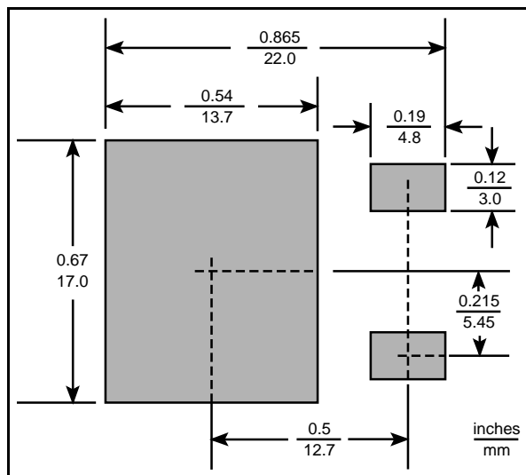
Figure 1. Minimum Recommended Footprint for the D 3 PAK.
