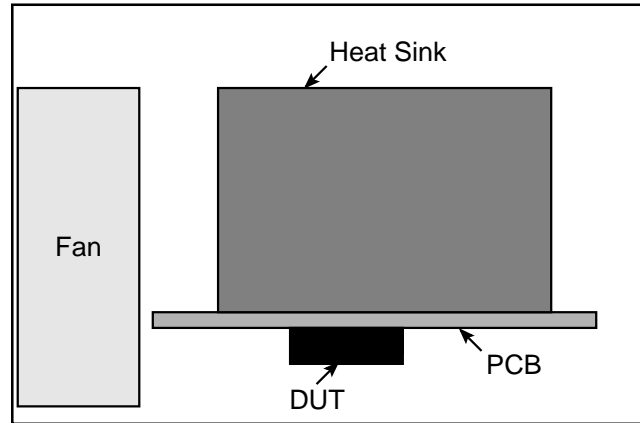
Figure 7. PCB With Forced Air on Heat Sink and device.
