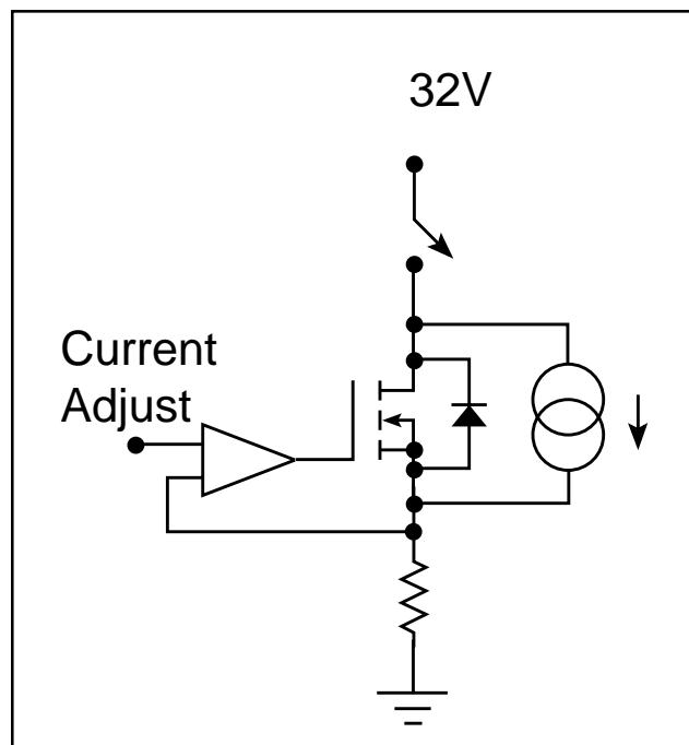
Figure 3. Simplified Test Setup Schematic.
