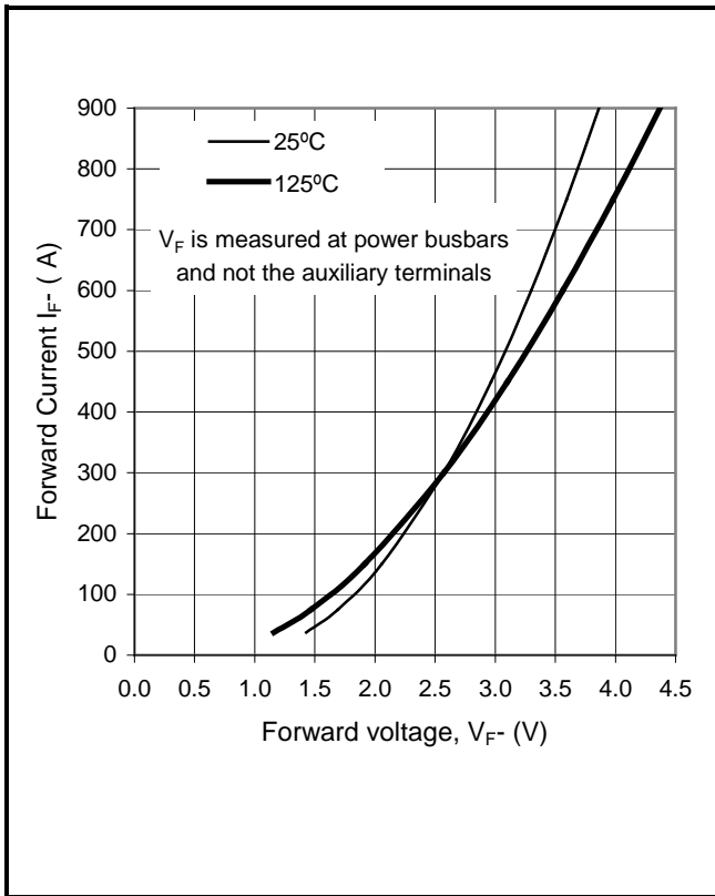
Fig.3 Diode typical forward characteristics
