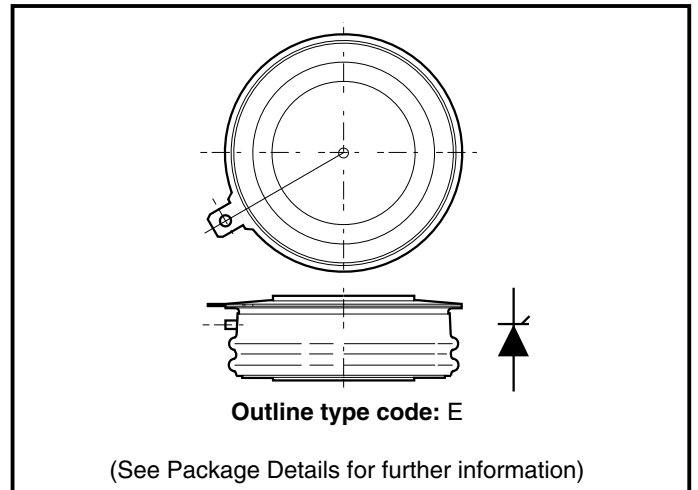
Fig. 1 Package outline
