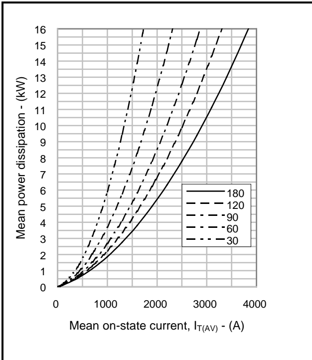
Fig.3 On-state power dissipation – sine wave
