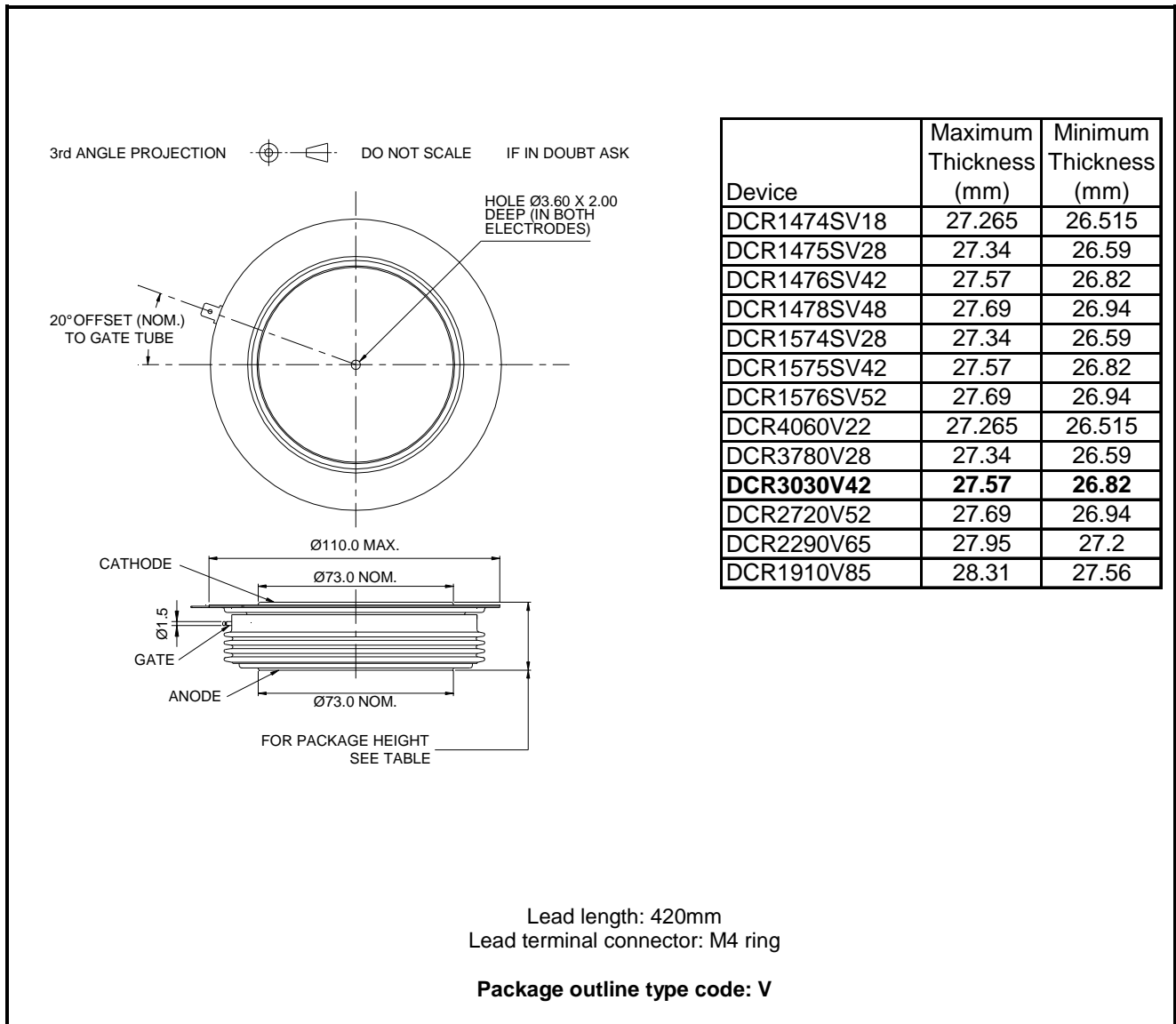
Fig.15 Package outline
