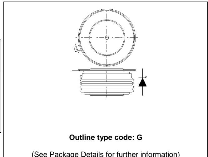
Fig. 1 Package outline
