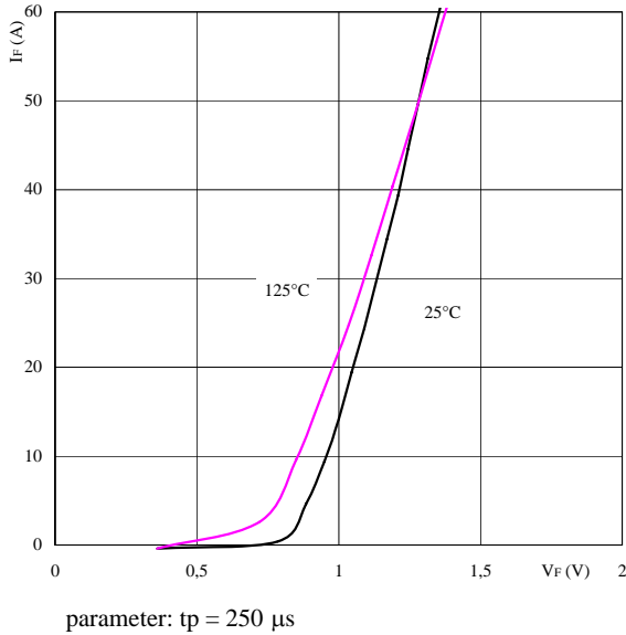
Figure 19. Typical diode forward current as a function of forward voltage
